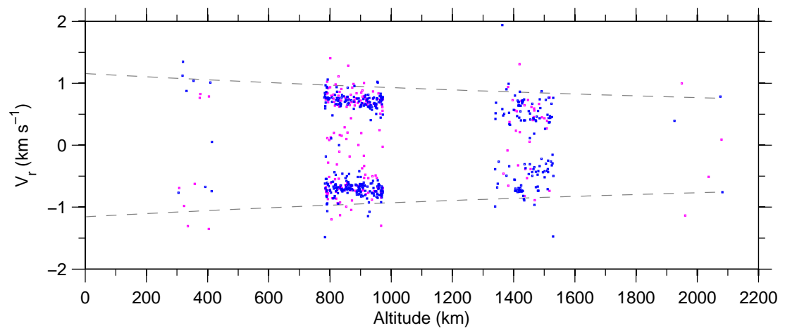
Figure 7: Doppler-velocity v altitude on 01-May-2007.
