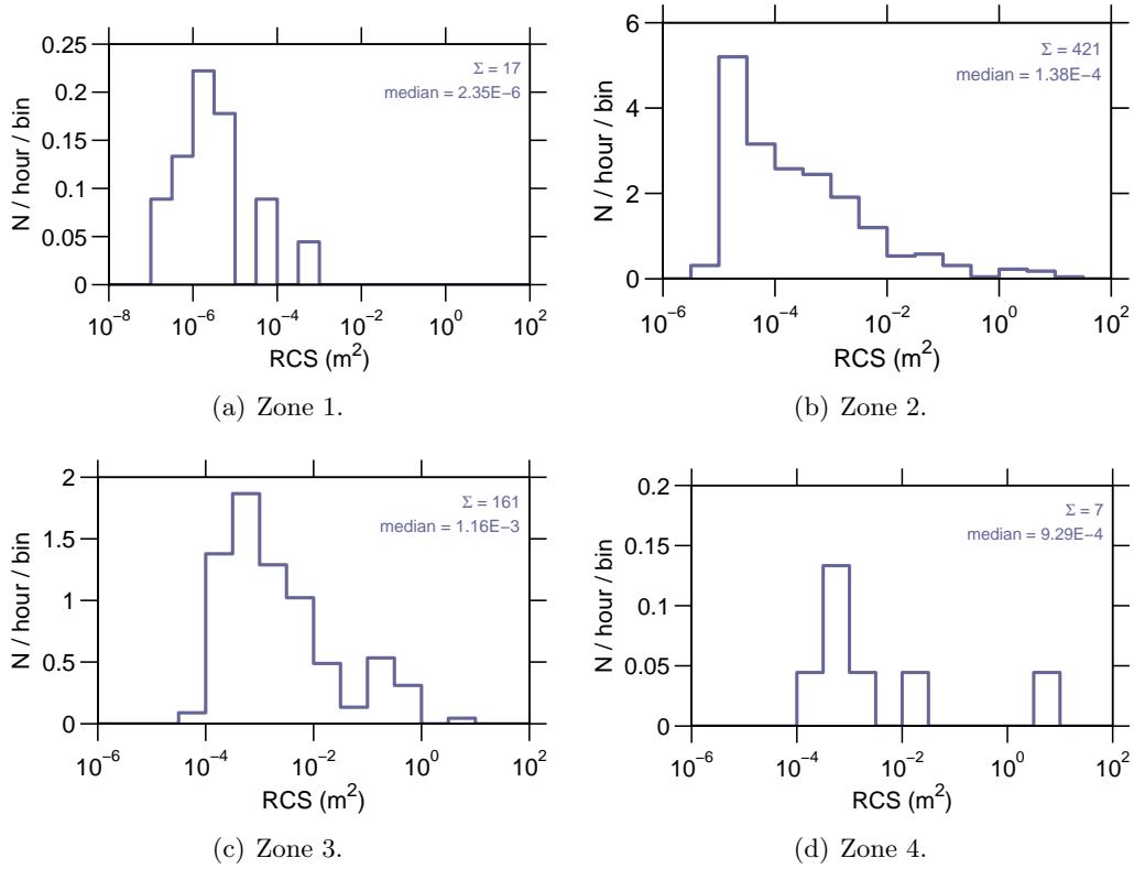
Figure 9: Event rate v RCS on 01-May-2007.
