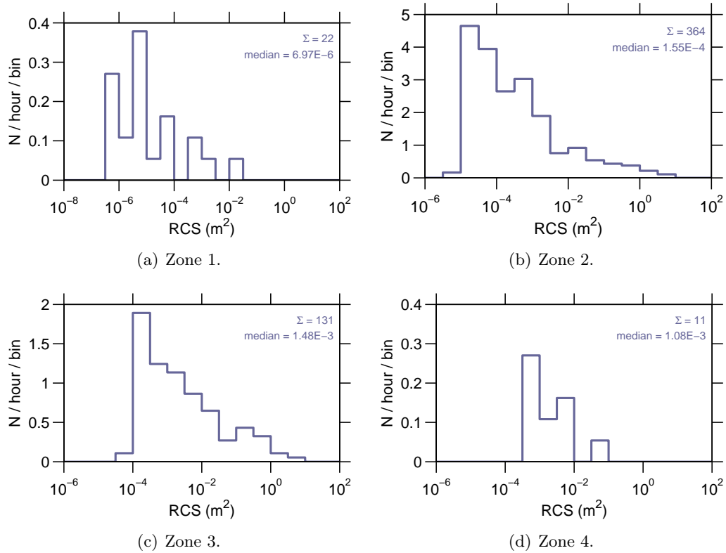
Figure 9: Event rate v RCS on 19-April-2007.
