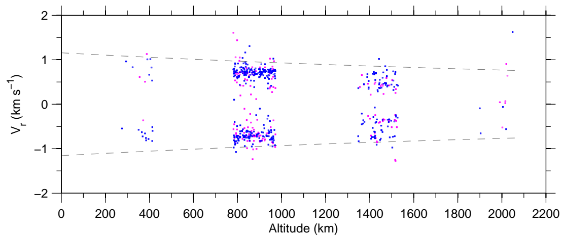
Figure 7: Doppler-velocity v altitude on 19-April-2007.
