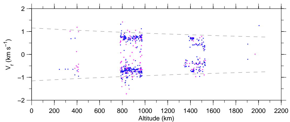
Figure 7: Doppler-velocity v altitude on 15-April-2007.
