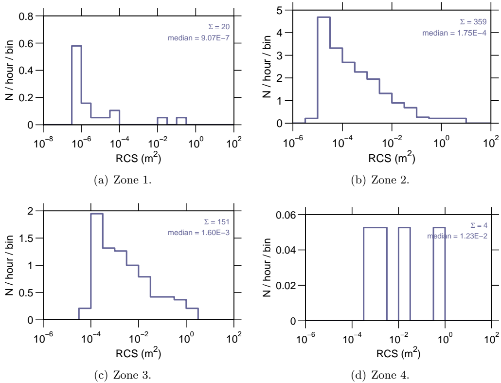
Figure 9: Event rate v RCS on 15-April-2007.
