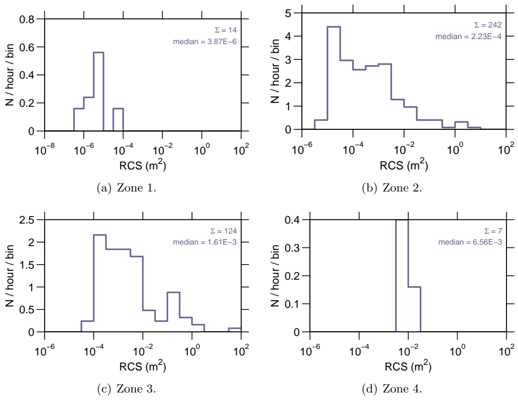
Figure 9: Event rate v RCS on 10-April-2007.
