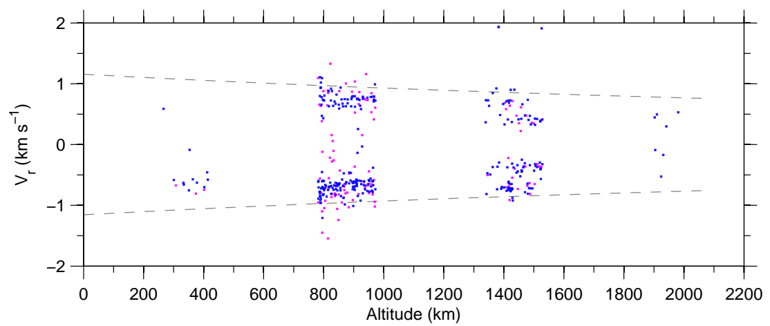
Figure 7: Doppler-velocity v altitude on 10-April-2007.
