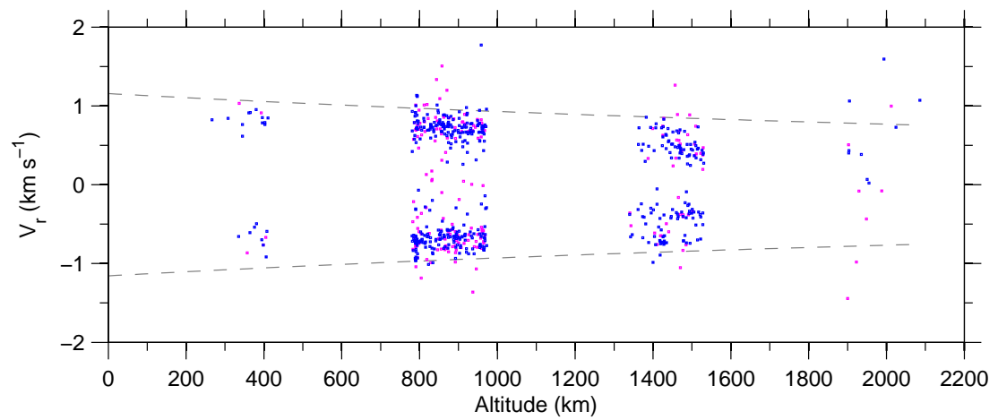
Figure 7: Doppler-velocity v altitude on 09-April-2007.
