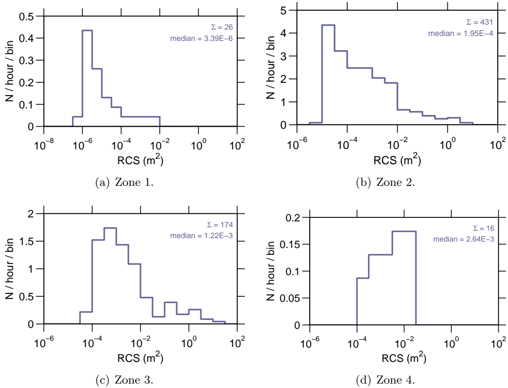
Figure 9: Event rate v RCS on 09-April-2007.
