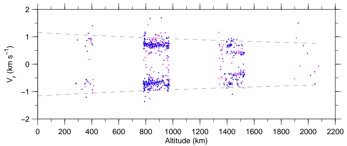
Figure 7: Doppler-velocity v altitude on 08-April-2007.
