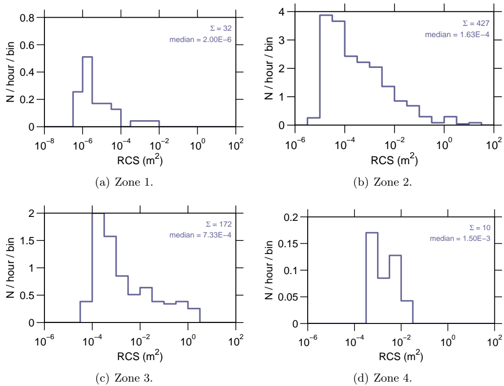
Figure 9: Event rate v RCS on 08-April-2007.
