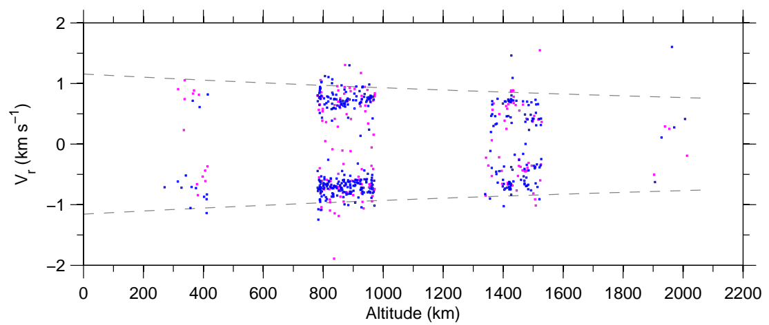
Figure 7: Doppler-velocity v altitude on 05-April-2007.
