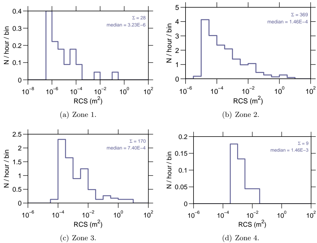
Figure 9: Event rate v RCS on 05-April-2007.
