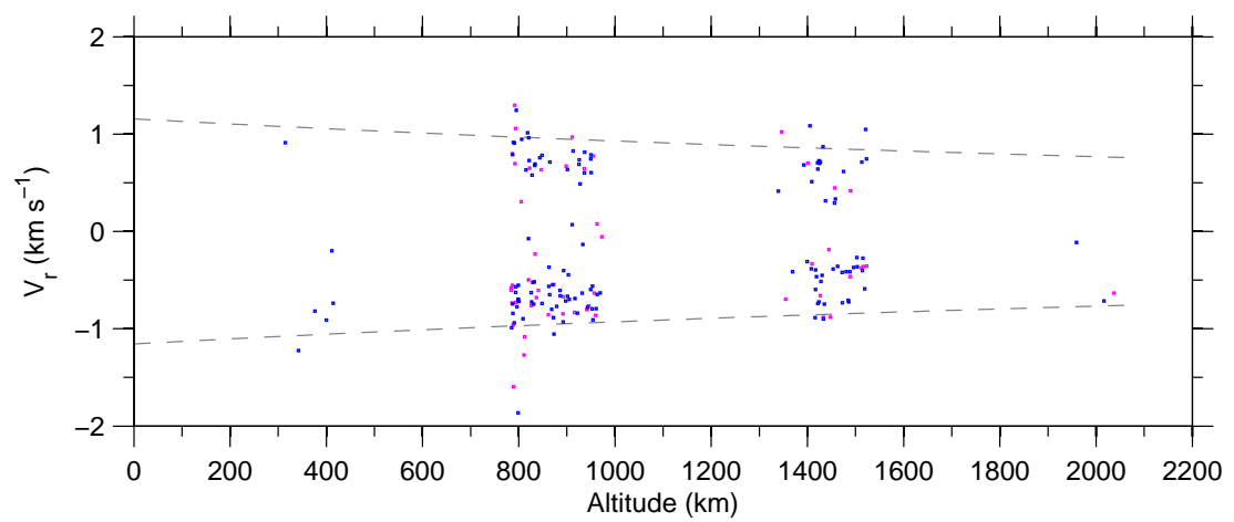
Figure 7: Doppler-velocity v altitude on 30-March-2007.
