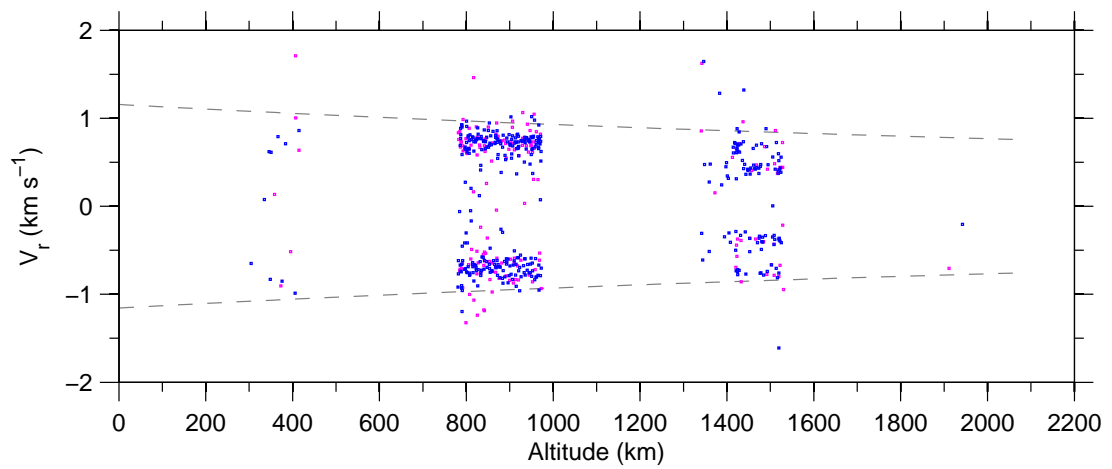
Figure 7: Doppler-velocity v altitude on 16-March-2007.
