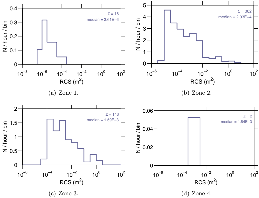
Figure 9: Event rate v RCS on 16-March-2007.
