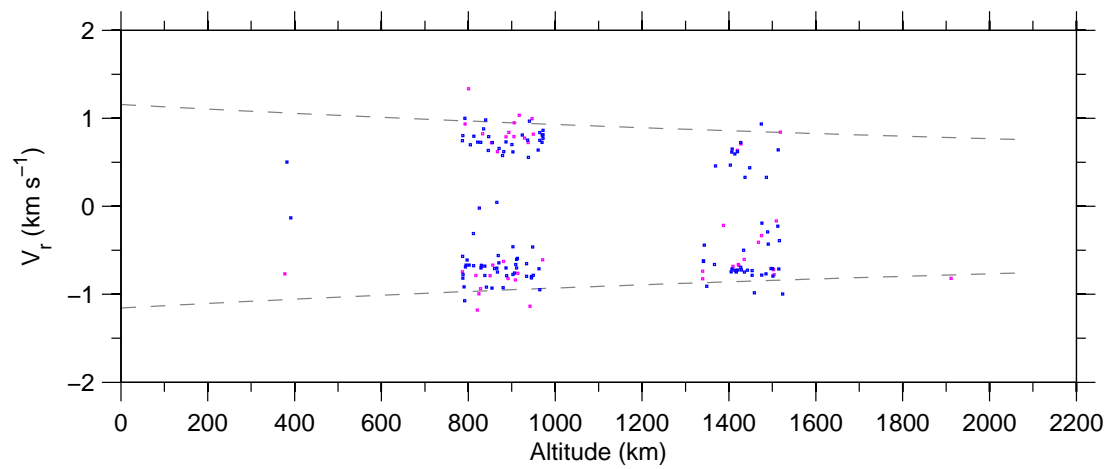
Figure 7: Doppler-velocity v altitude on 11-March-2007.
