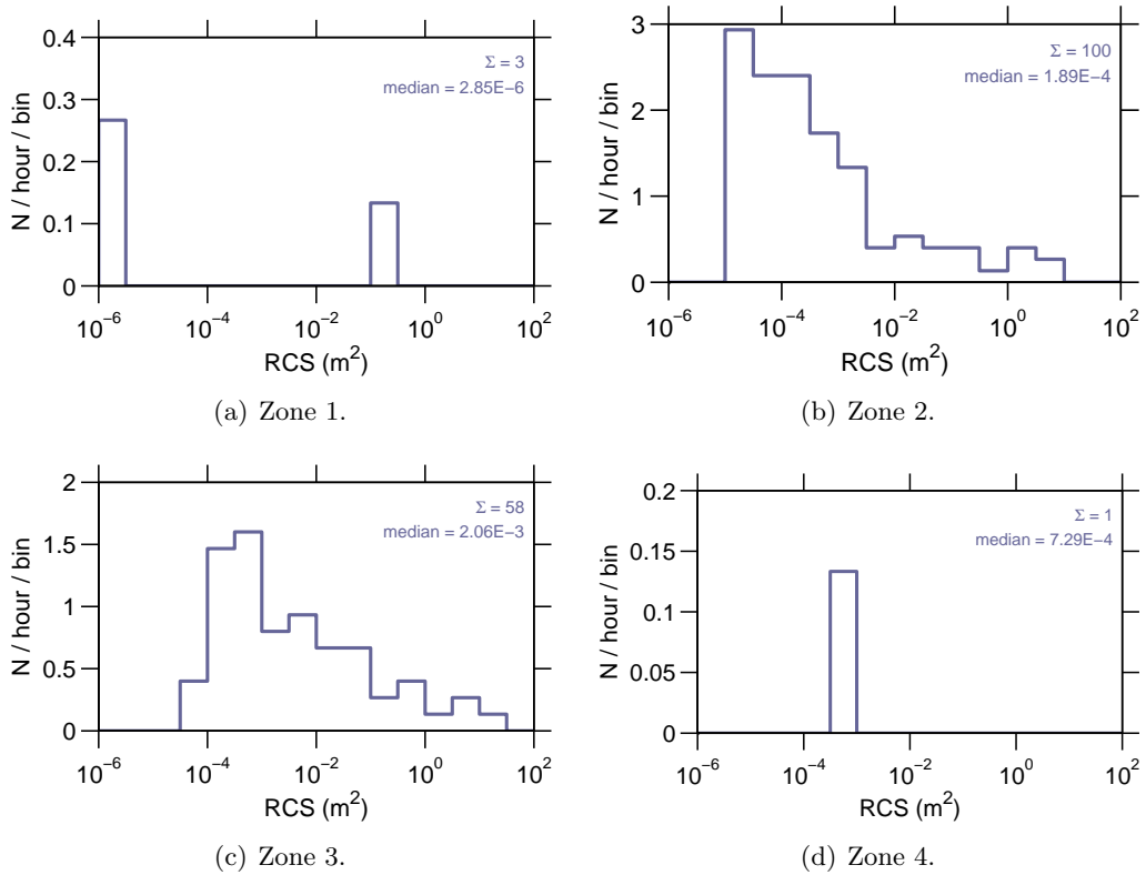
Figure 9: Event rate v RCS on 11-March-2007.
